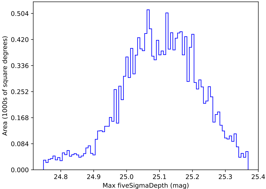
noroll_mjdp120_v3.4_10yrs WFD all bands: Max fiveSigmaDepth
