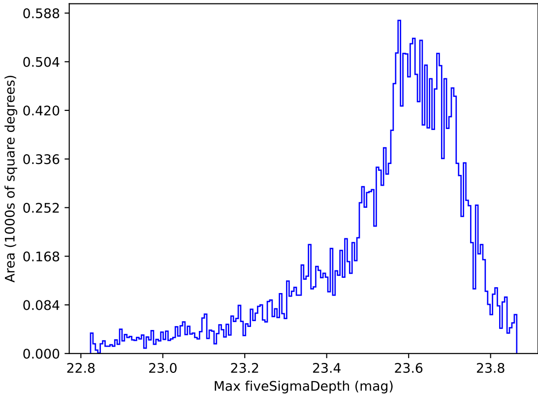
noroll_mjdp120_v3.4_10yrs All sky z band: Max fiveSigmaDepth
