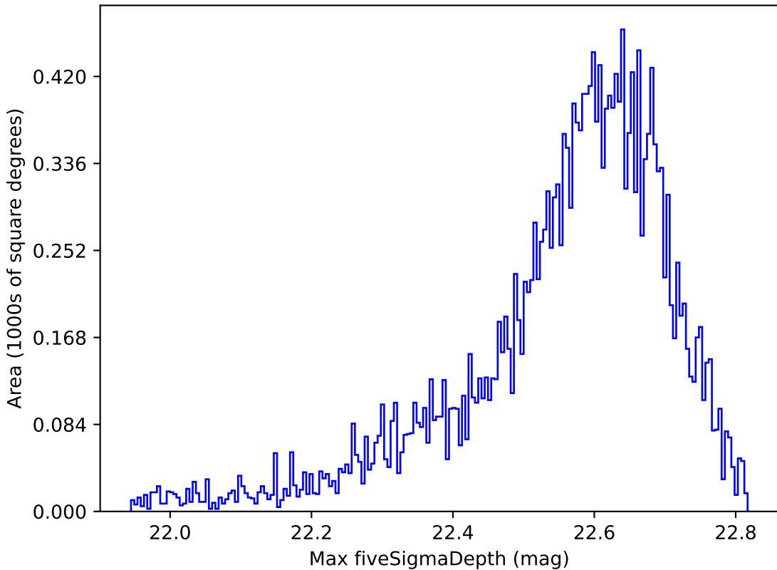
noroll_mjdp120_v3.4_10yrs All sky y band: Max fiveSigmaDepth
