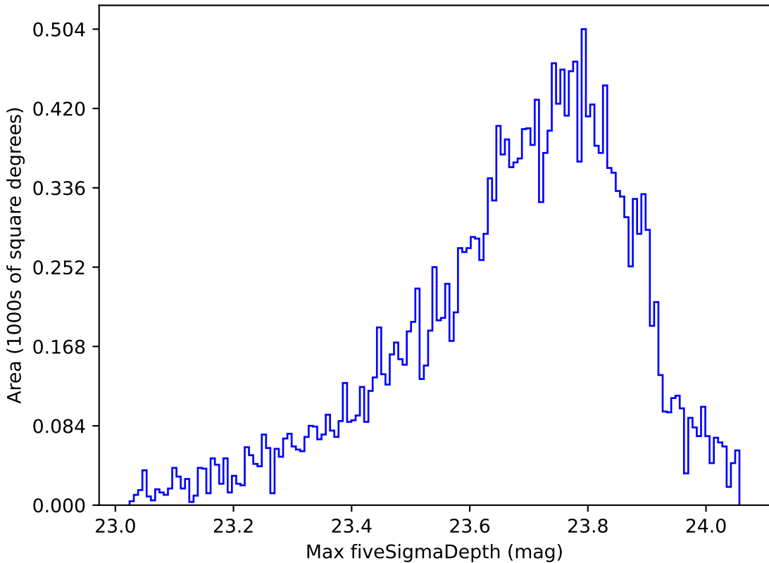
noroll_mjdp120_v3.4_10yrs All sky u band: Max fiveSigmaDepth
