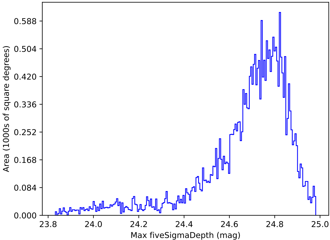
noroll_mjdp120_v3.4_10yrs All sky r band: Max fiveSigmaDepth
