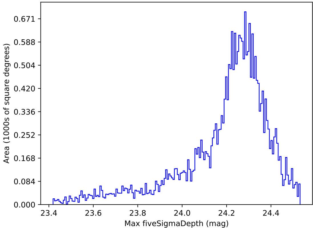
noroll_mjdp120_v3.4_10yrs All sky i band: Max fiveSigmaDepth
