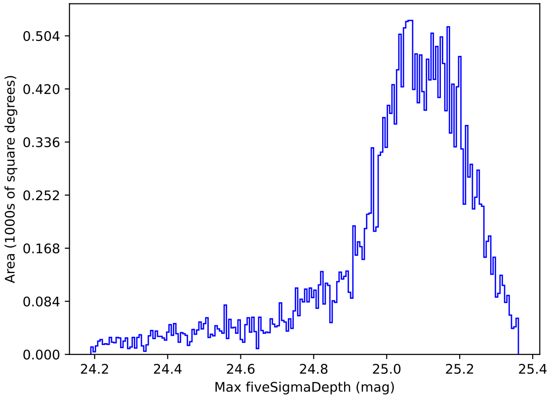
noroll_mjdp120_v3.4_10yrs All sky g band: Max fiveSigmaDepth
