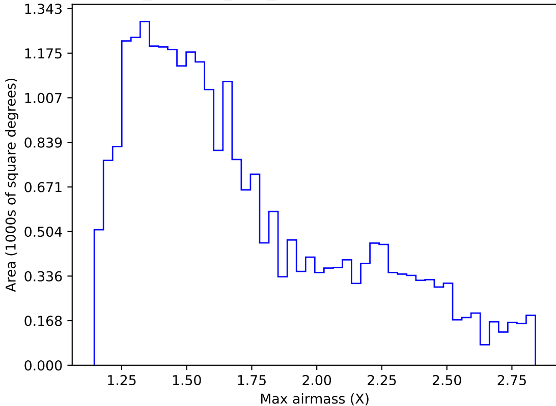
noroll_mjdp120_v3.4_10yrs Yr 1 z band: Max airmass
