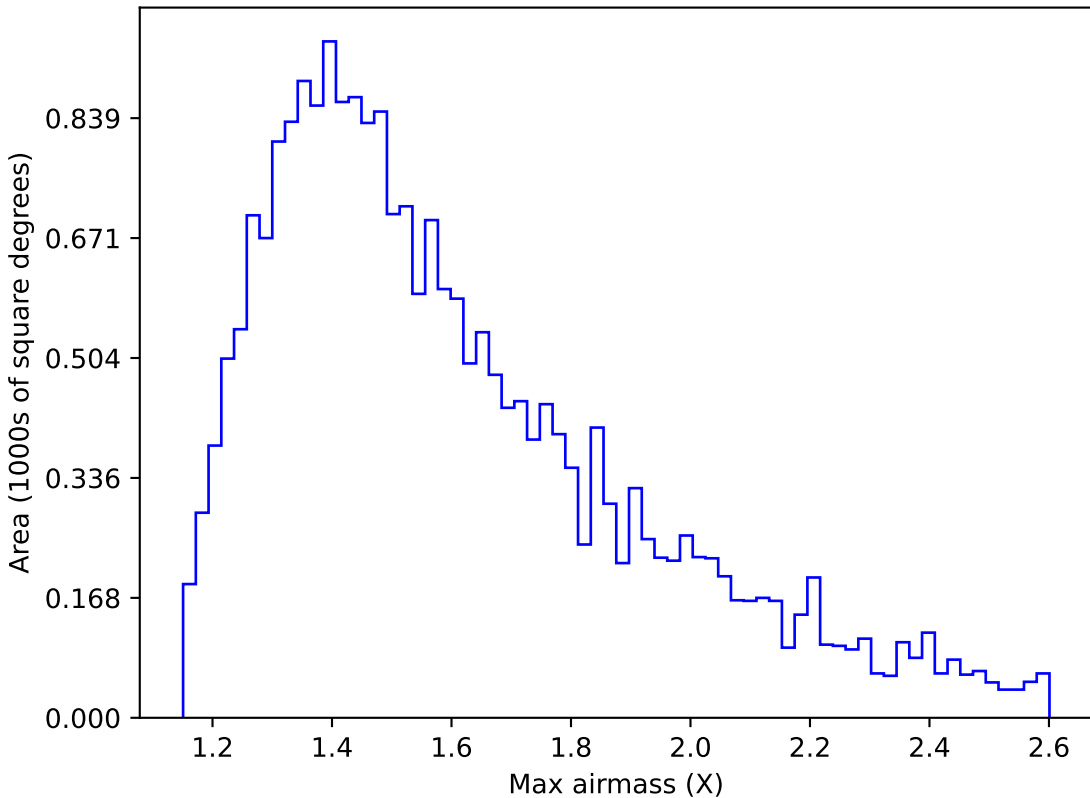
noroll_mjdp120_v3.4_10yrs Yr 1 y band: Max airmass
