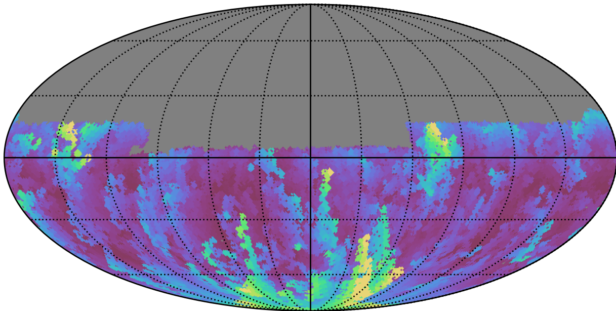
noroll_mjdp120_v3.4_10yrs Yr 1 u band: Max airmass
