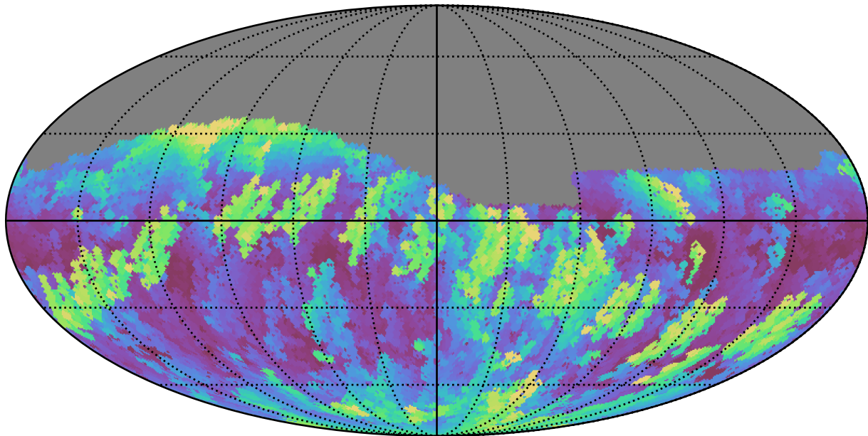
noroll_mjdp120_v3.4_10yrs Yr 1 r band: Max airmass
