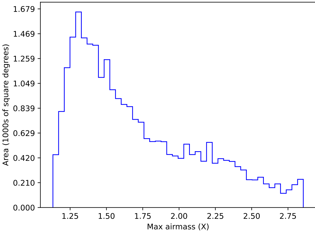
noroll_mjdp120_v3.4_10yrs Yr 1 i band: Max airmass
