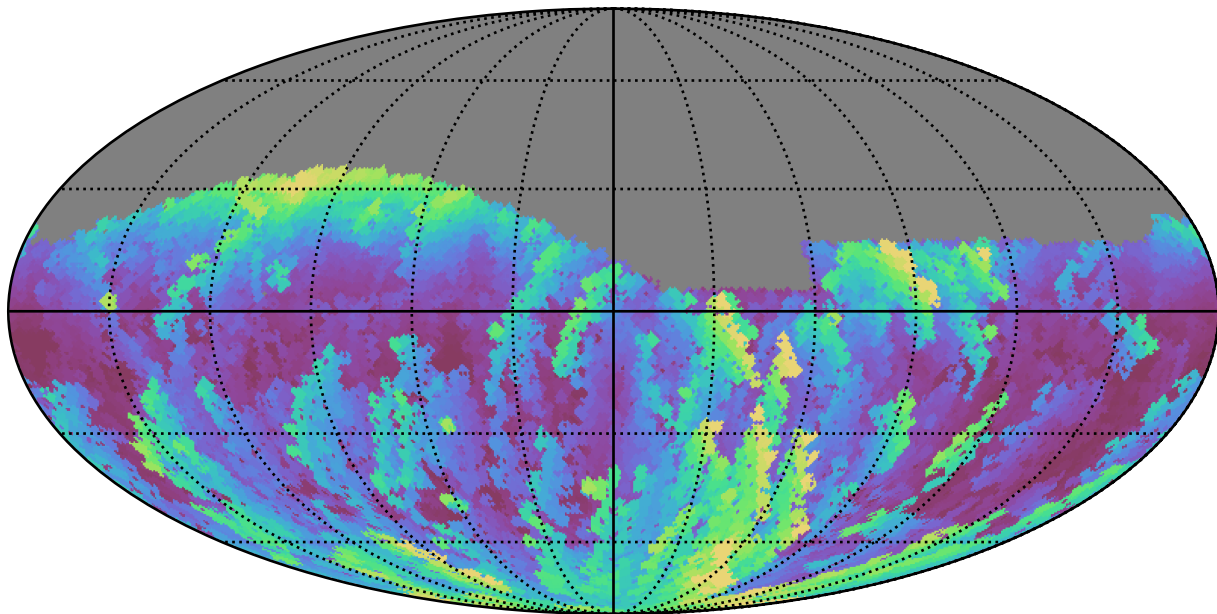
noroll_mjdp120_v3.4_10yrs Yr 1 g band: Max airmass
