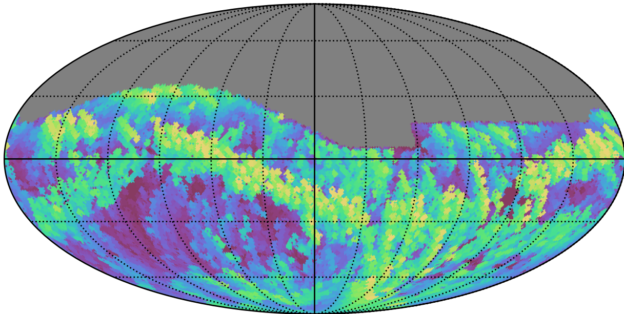
noroll_mjdp120_v3.4_10yrs Yr 1 all bands: Max airmass
