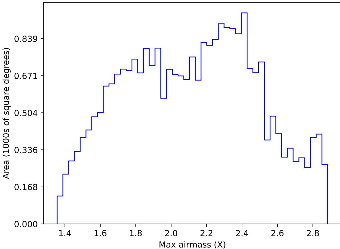
noroll_mjdp120_v3.4_10yrs Yr 1 all bands: Max airmass
