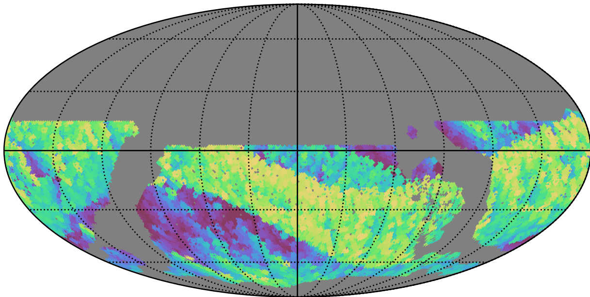
noroll_mjdp120_v3.4_10yrs WFD z band: Max airmass
