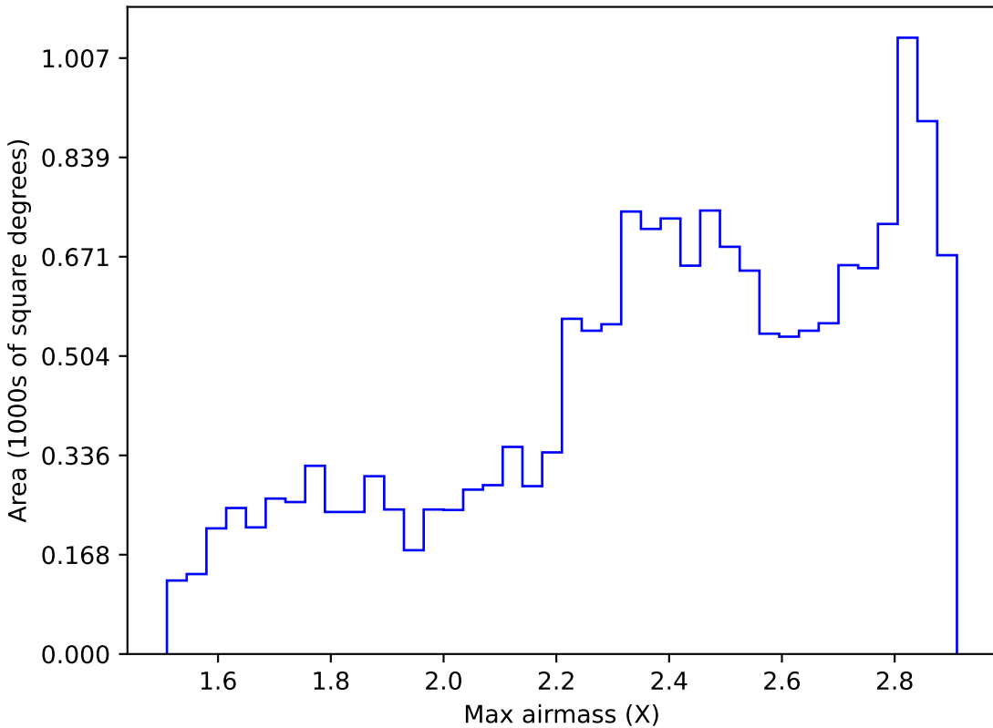
noroll_mjdp120_v3.4_10yrs WFD z band: Max airmass
