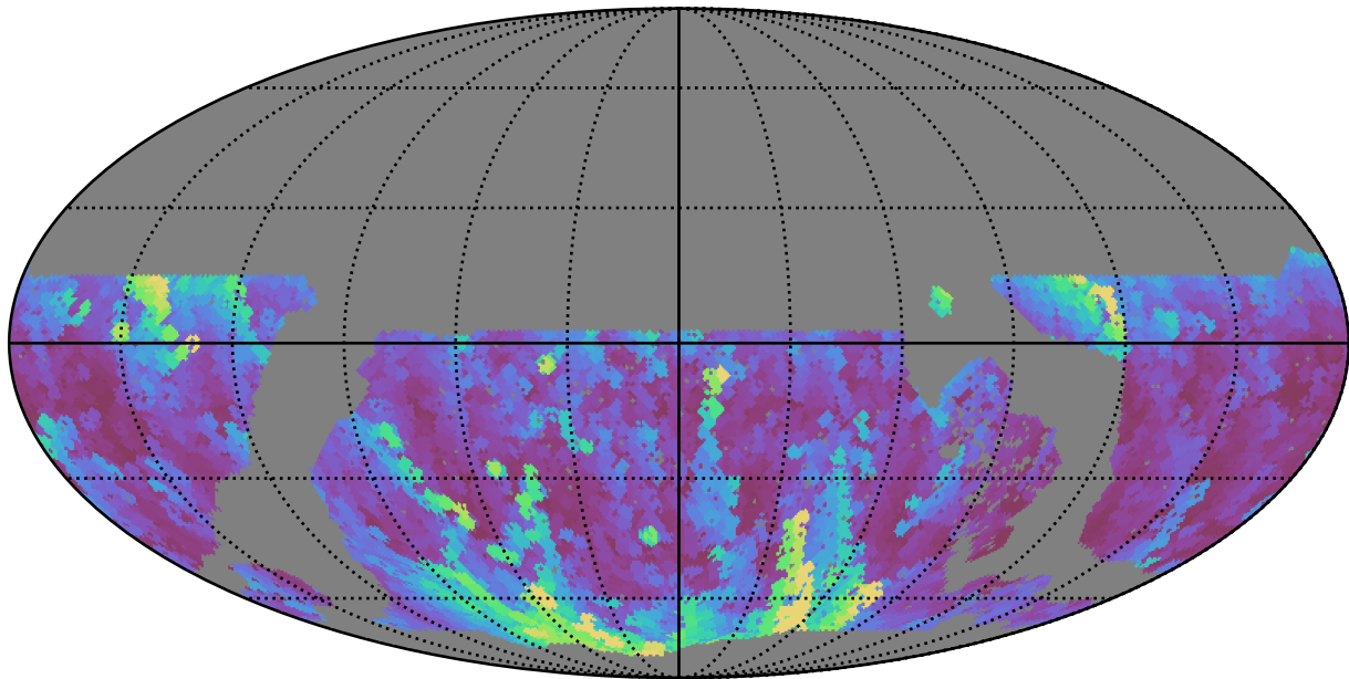
noroll_mjdp120_v3.4_10yrs WFD u band: Max airmass
