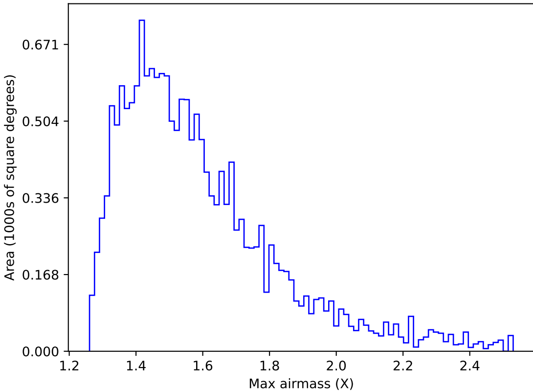
noroll_mjdp120_v3.4_10yrs WFD u band: Max airmass
