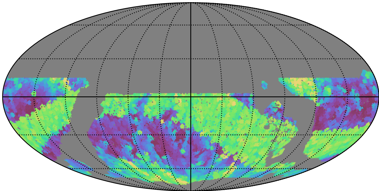
noroll_mjdp120_v3.4_10yrs WFD r band: Max airmass
