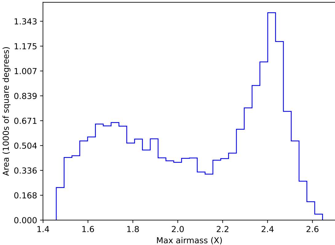
noroll_mjdp120_v3.4_10yrs WFD r band: Max airmass
