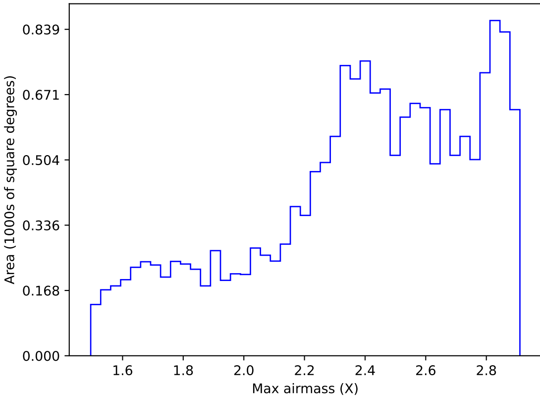
noroll_mjdp120_v3.4_10yrs WFD i band: Max airmass
