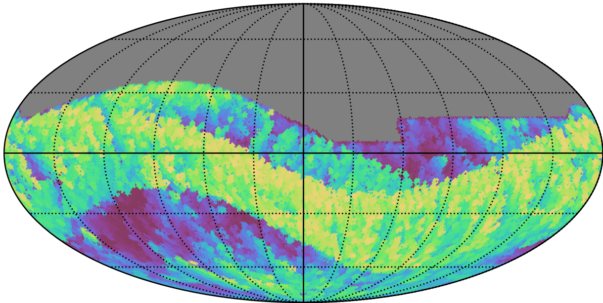
noroll_mjdp120_v3.4_10yrs All sky z band: Max airmass
