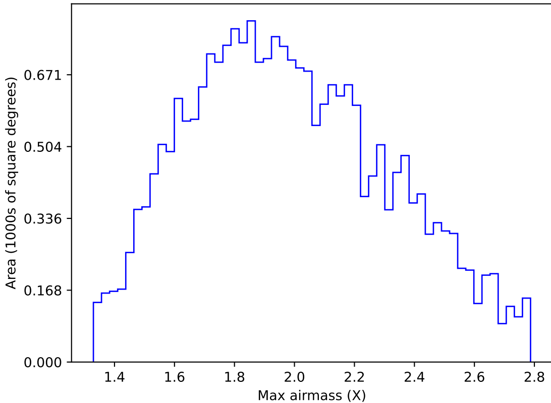
noroll_mjdp120_v3.4_10yrs All sky y band: Max airmass
