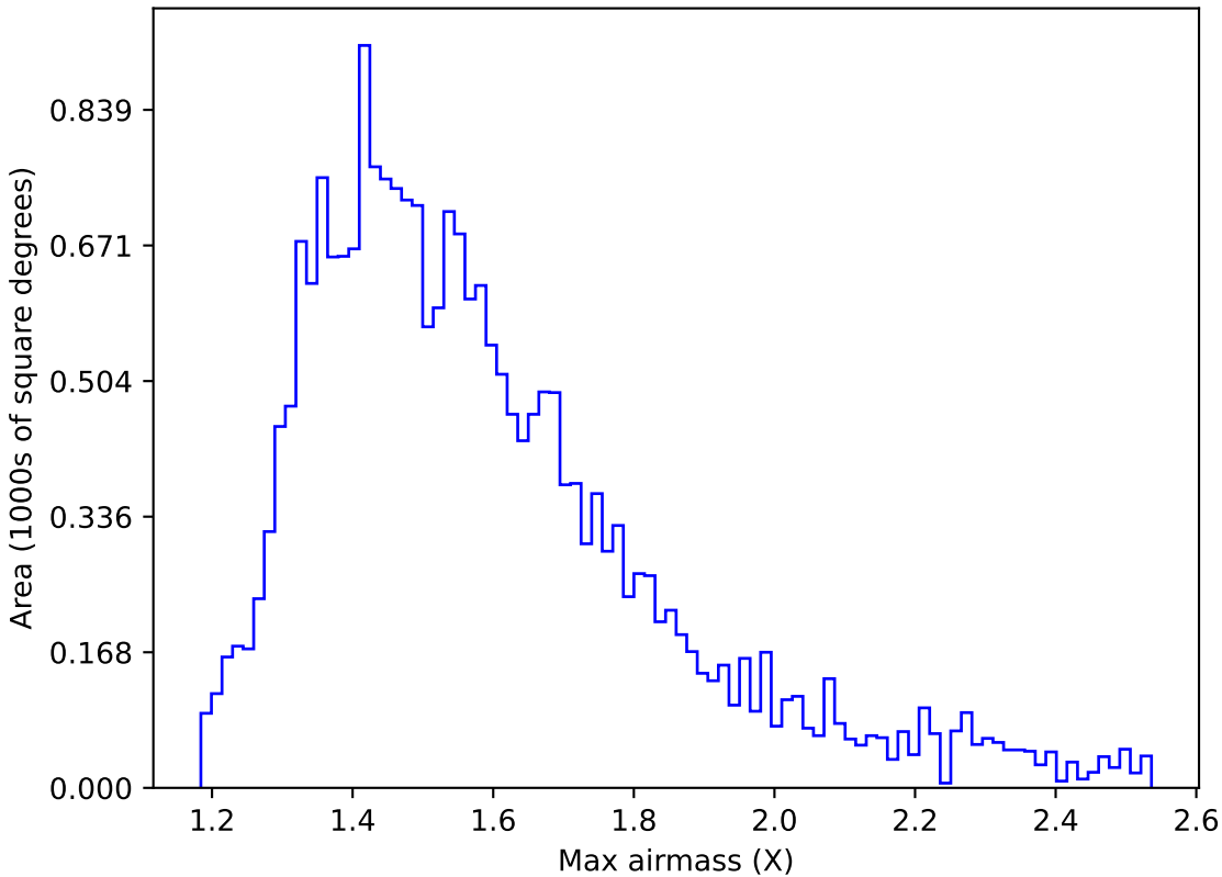
noroll_mjdp120_v3.4_10yrs All sky u band: Max airmass
