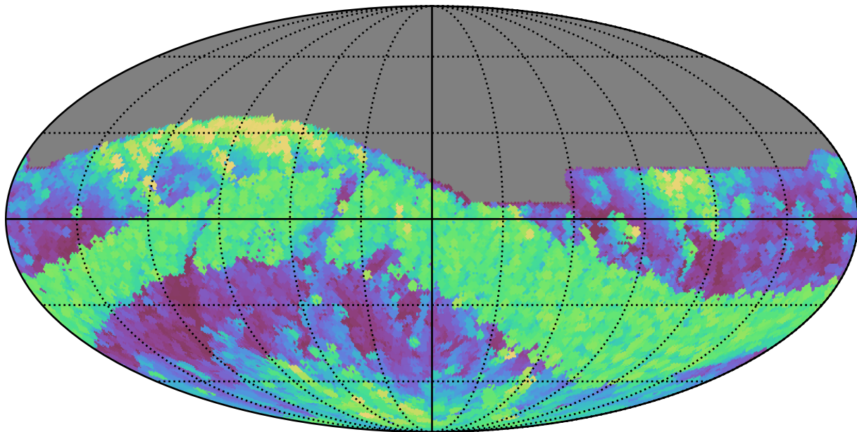
noroll_mjdp120_v3.4_10yrs All sky r band: Max airmass
