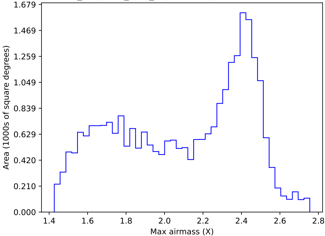
noroll_mjdp120_v3.4_10yrs All sky r band: Max airmass
