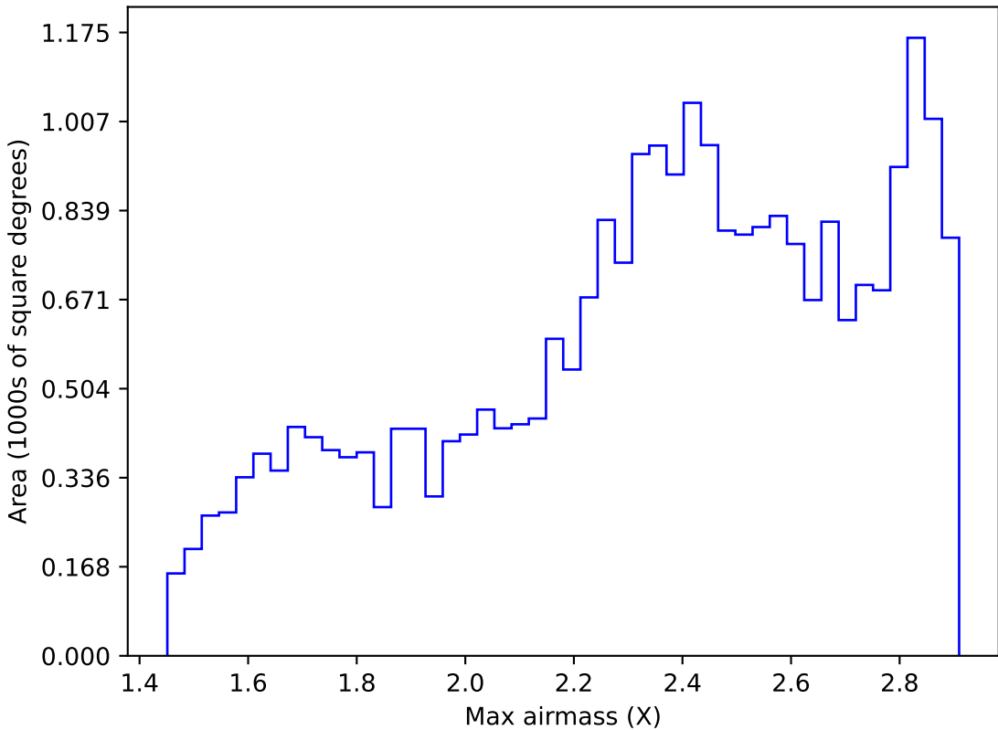
noroll_mjdp120_v3.4_10yrs All sky i band: Max airmass
