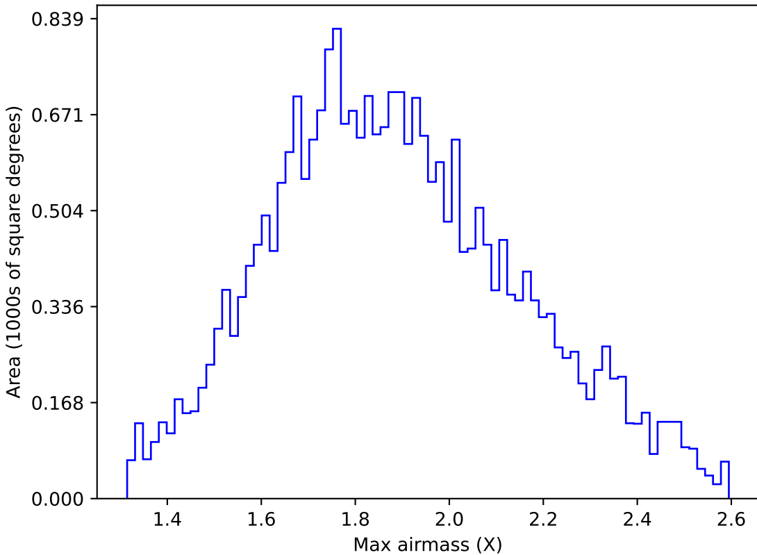
noroll_mjdp120_v3.4_10yrs All sky g band: Max airmass
