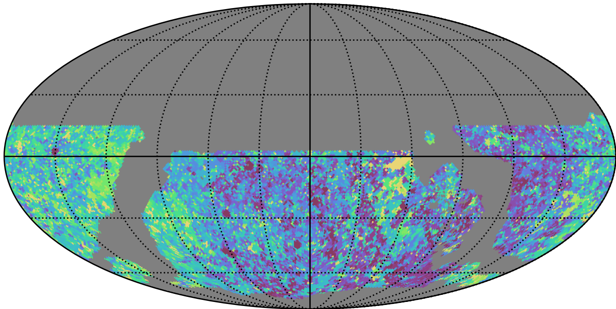
noroll_mjdp120_v3.4_10yrs WFD z band: Max Inter-Night Gap
