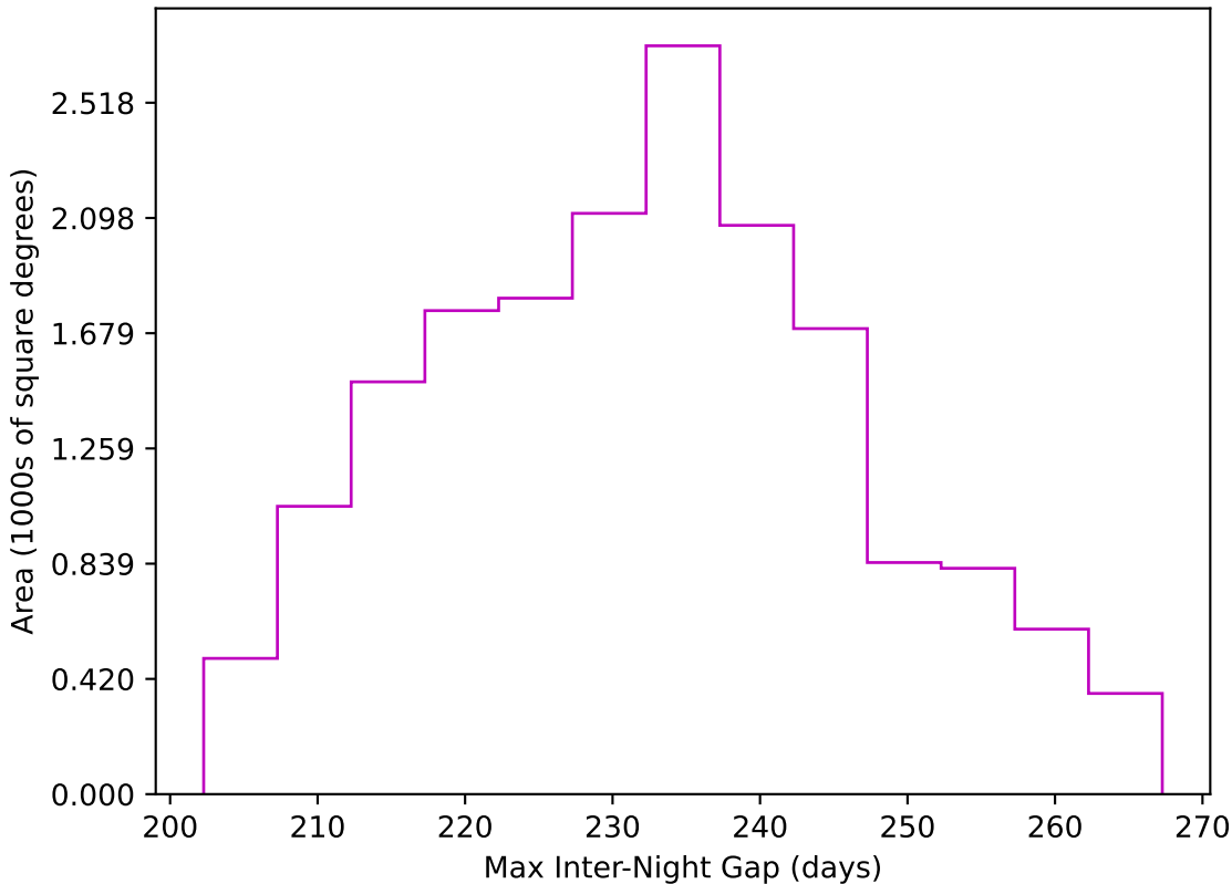
noroll_mjdp120_v3.4_10yrs WFD z band: Max Inter-Night Gap
