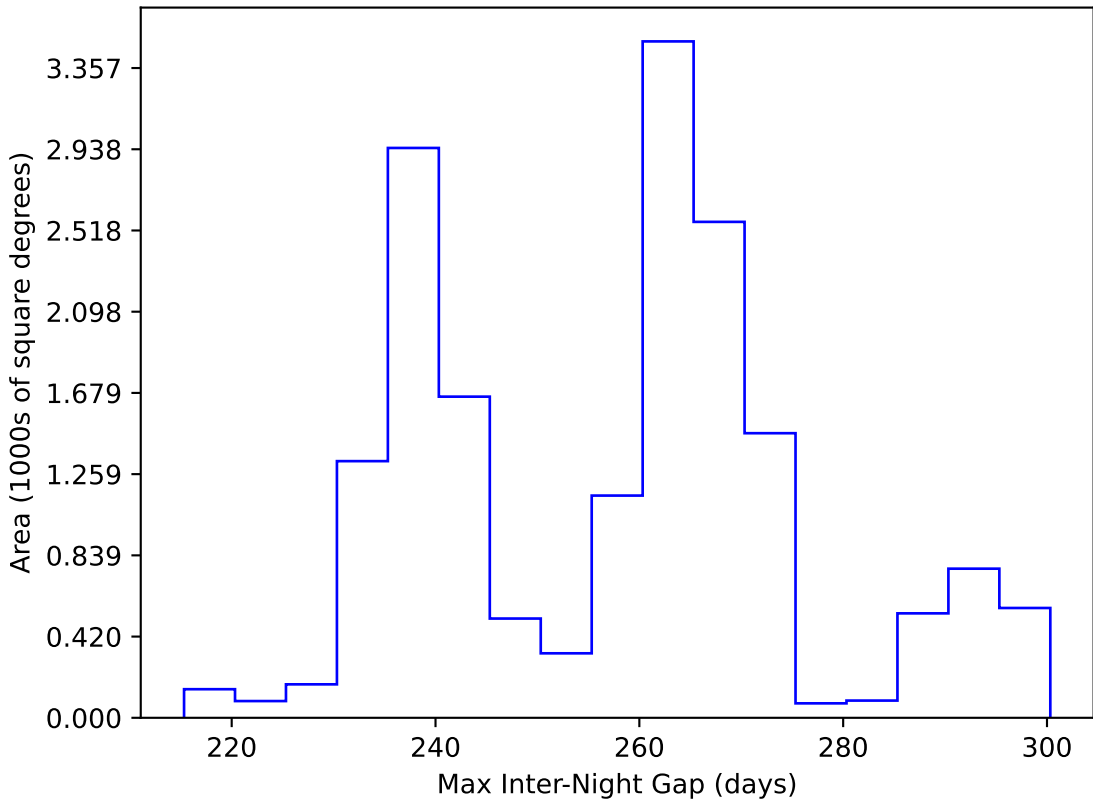
noroll_mjdp120_v3.4_10yrs WFD y band: Max Inter-Night Gap
