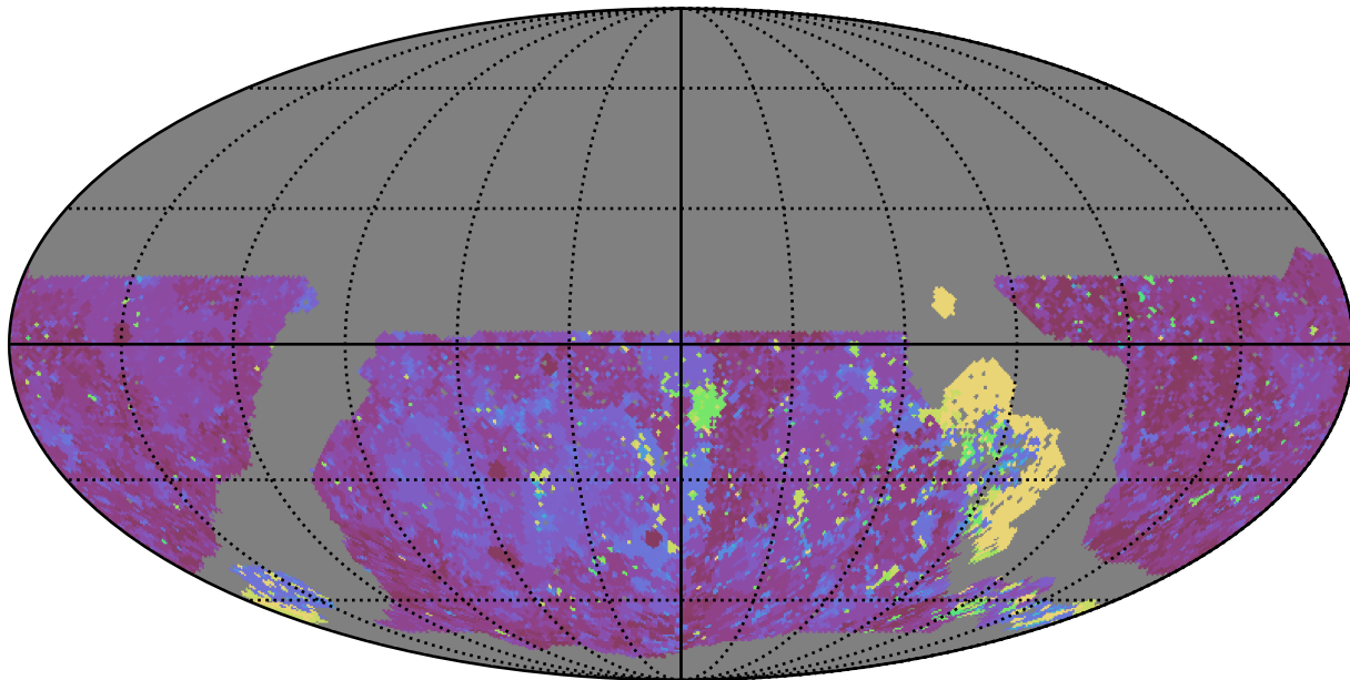
noroll_mjdp120_v3.4_10yrs WFD u band: Max Inter-Night Gap
