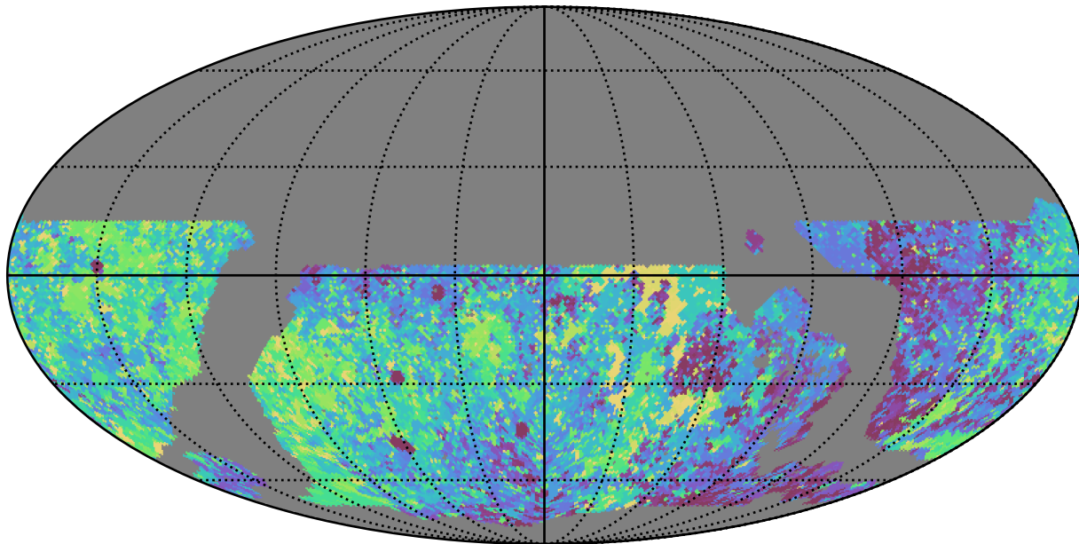
noroll_mjdp120_v3.4_10yrs WFD r band: Max Inter-Night Gap
