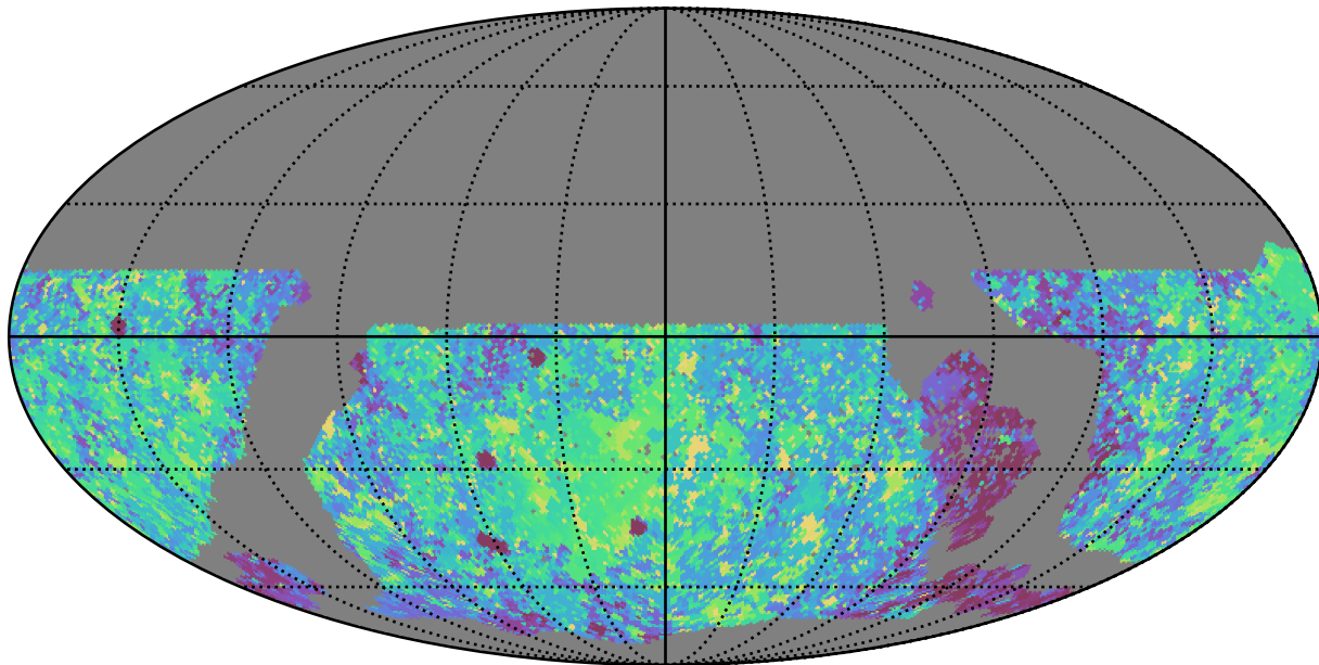
noroll_mjdp120_v3.4_10yrs WFD g band: Max Inter-Night Gap
