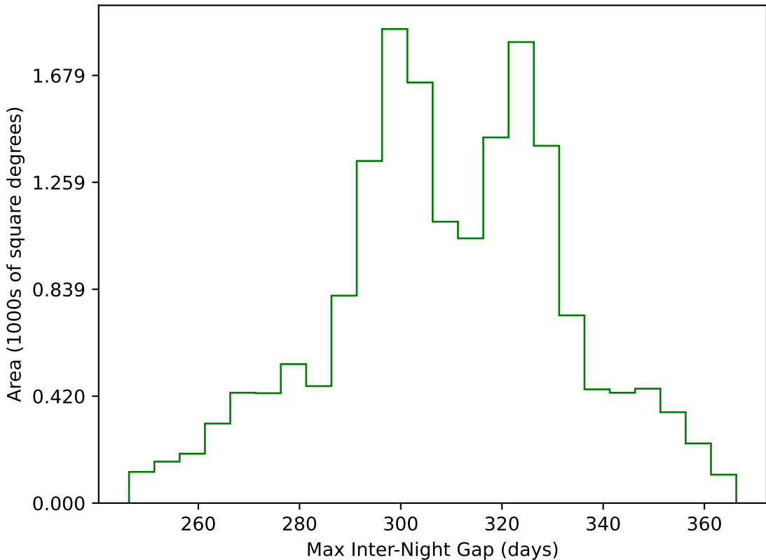
noroll_mjdp120_v3.4_10yrs WFD g band: Max Inter-Night Gap
