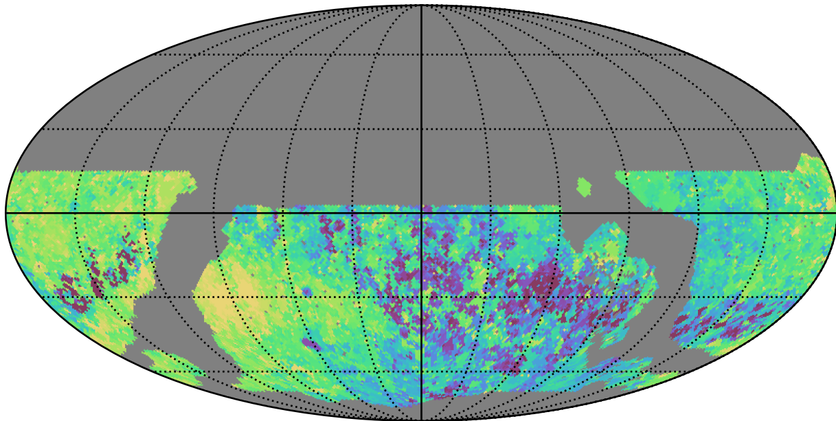
noroll_mjdp120_v3.4_10yrs WFD all bands: Max Inter-Night Gap
