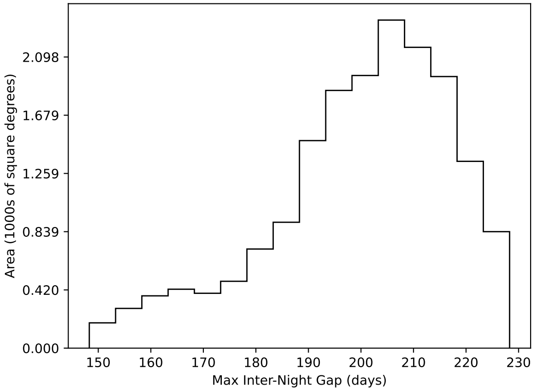
noroll_mjdp120_v3.4_10yrs WFD all bands: Max Inter-Night Gap
