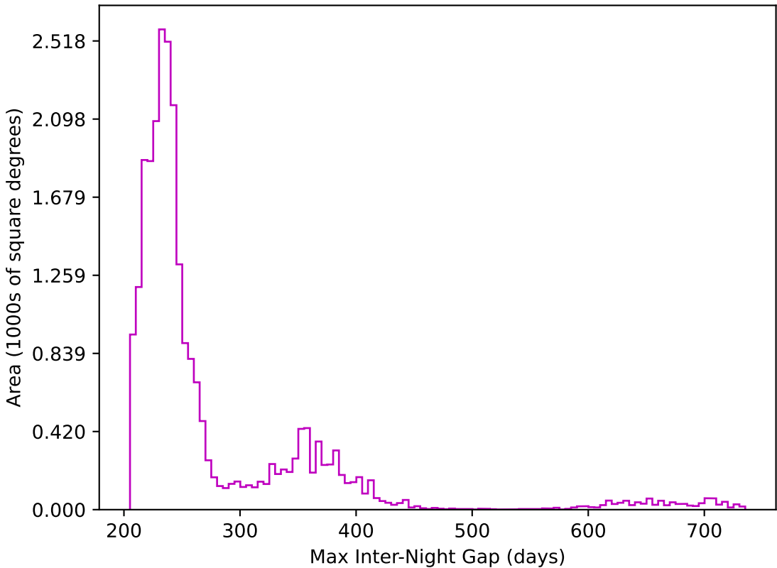
noroll_mjdp120_v3.4_10yrs All sky z band: Max Inter-Night Gap
