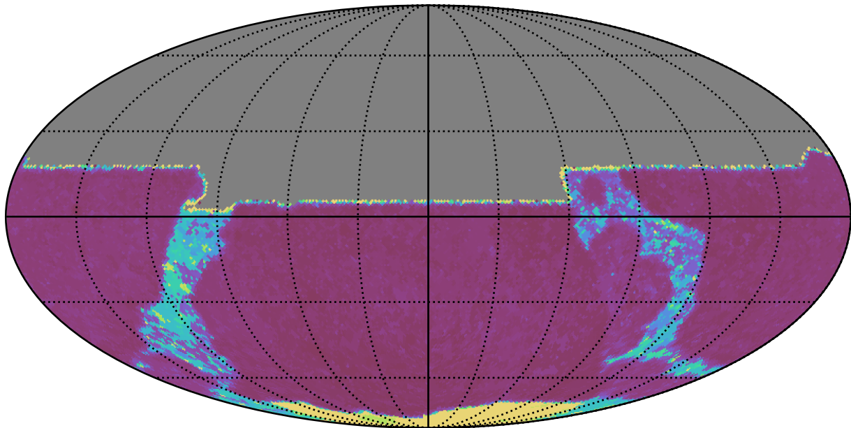
noroll_mjdp120_v3.4_10yrs All sky y band: Max Inter-Night Gap
