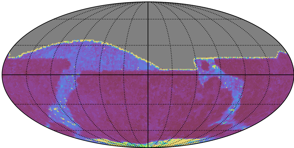
noroll_mjdp120_v3.4_10yrs All sky i band: Max Inter-Night Gap
