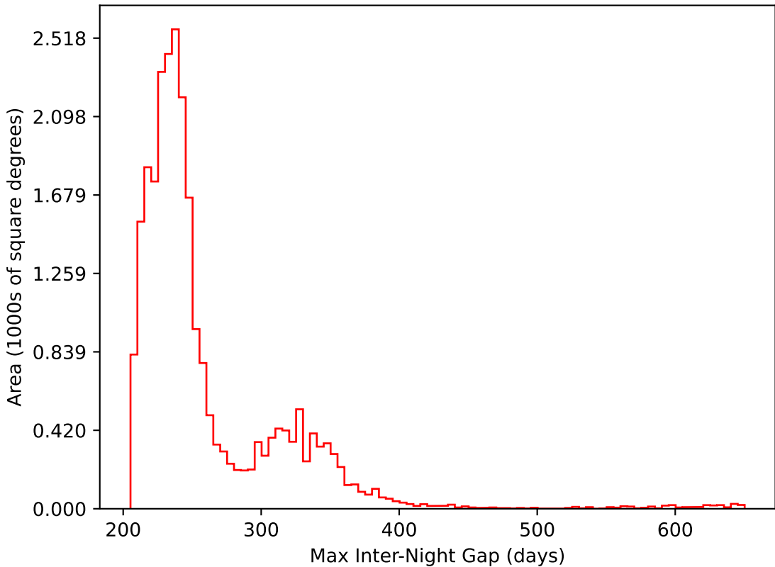
noroll_mjdp120_v3.4_10yrs All sky i band: Max Inter-Night Gap
