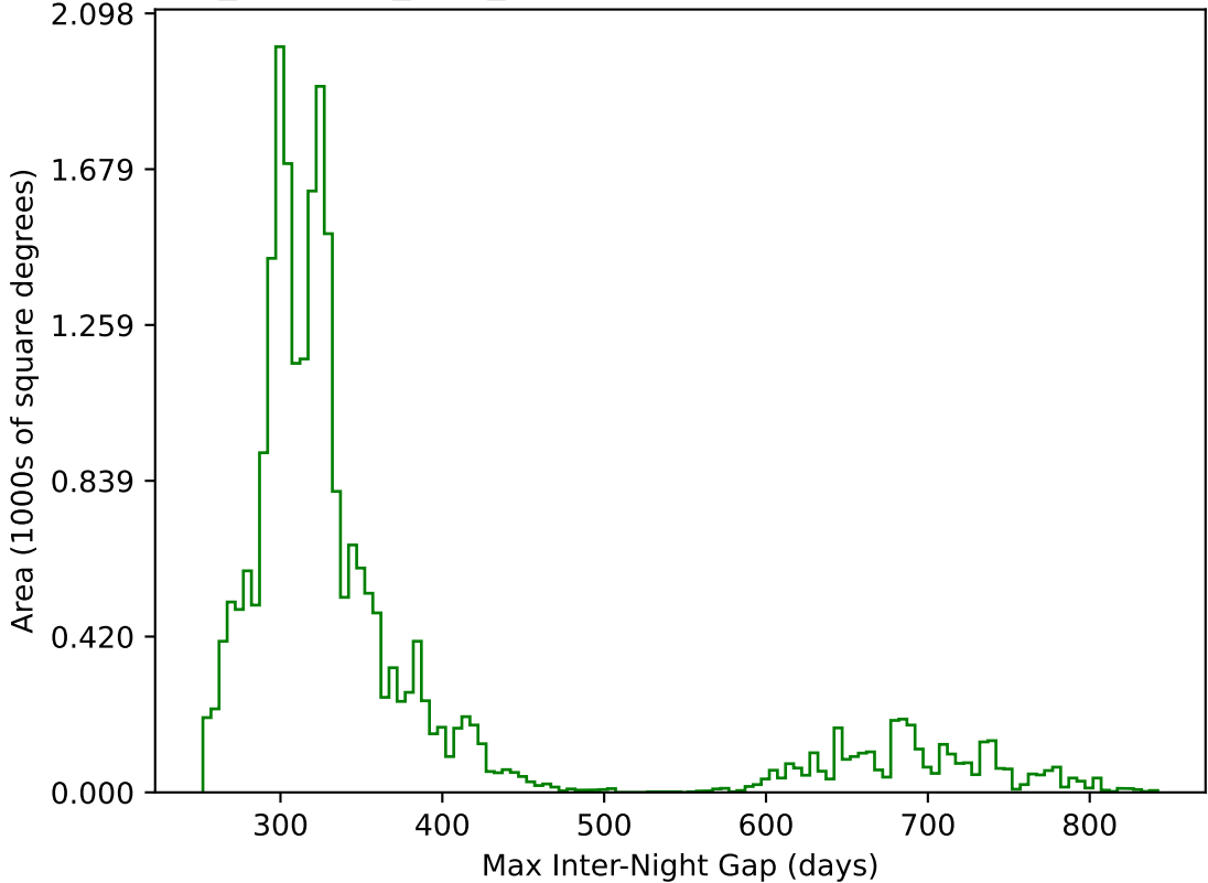
noroll_mjdp120_v3.4_10yrs All sky g band: Max Inter-Night Gap
