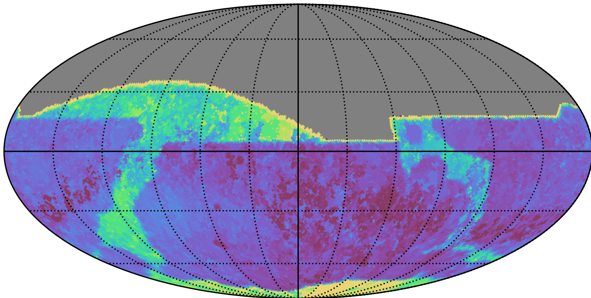
noroll_mjdp120_v3.4_10yrs All sky all bands: Max Inter-Night Gap
