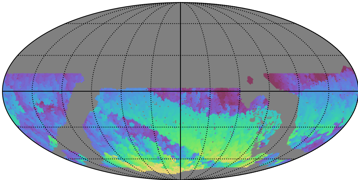
noroll_mjdp120_v3.4_10yrs WFD z band: Max HA
