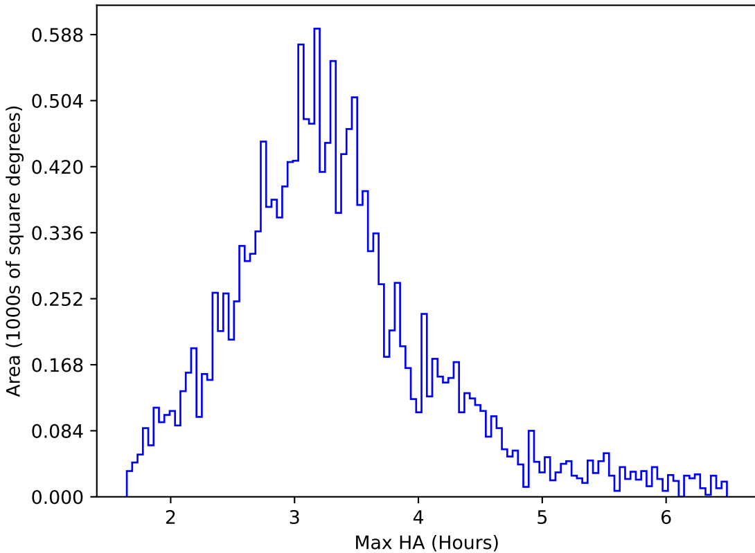
noroll_mjdp120_v3.4_10yrs WFD u band: Max HA
