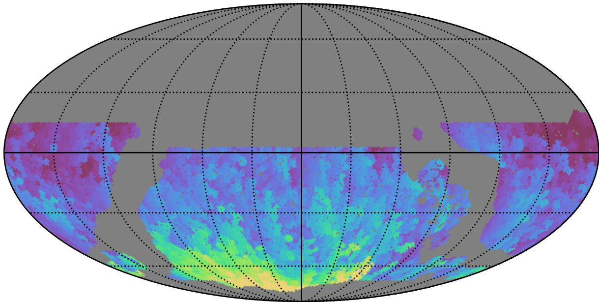
noroll_mjdp120_v3.4_10yrs WFD r band: Max HA
