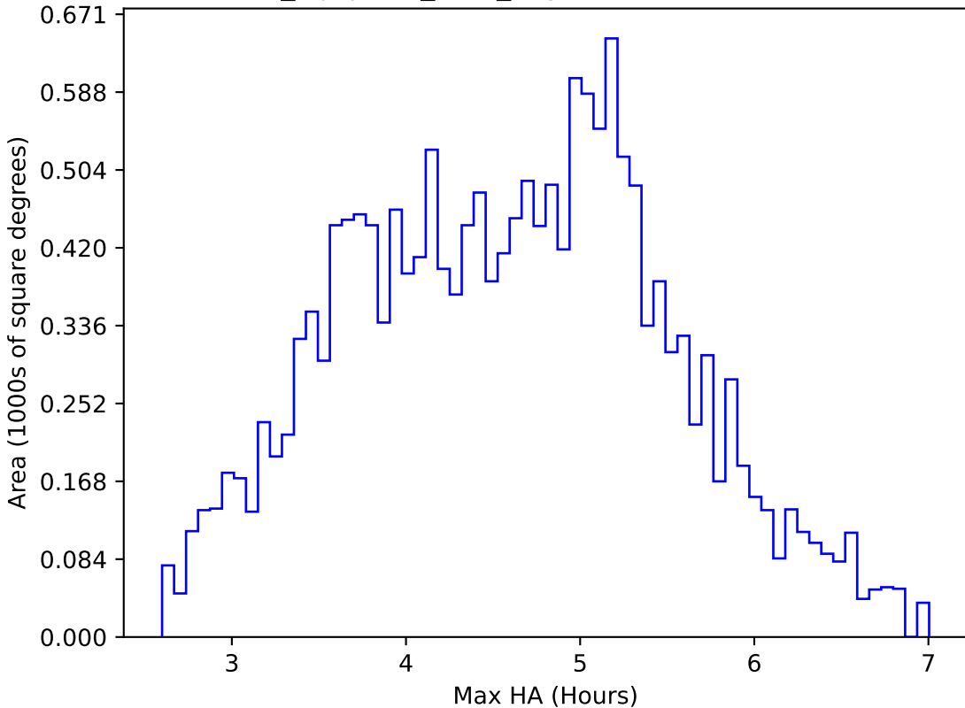
noroll_mjdp120_v3.4_10yrs WFD i band: Max HA
