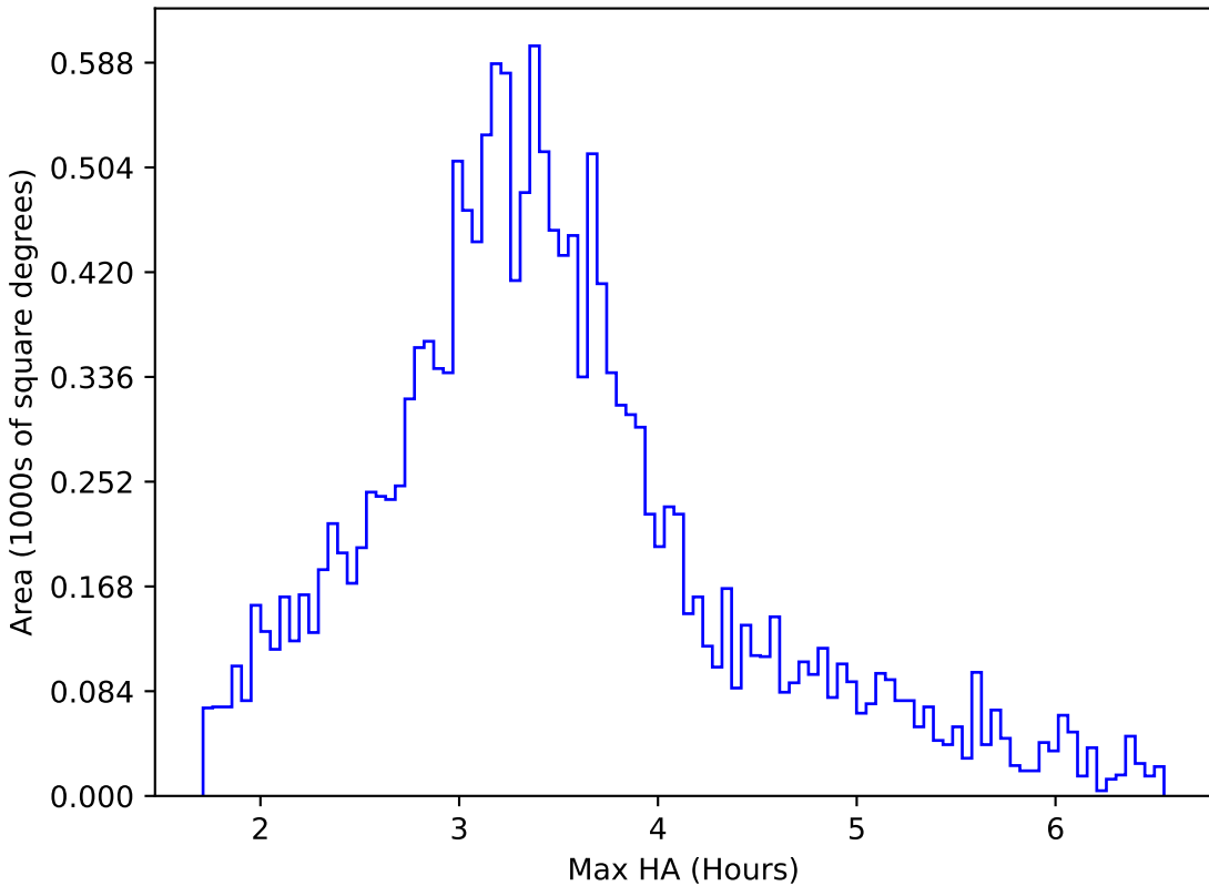
noroll_mjdp120_v3.4_10yrs WFD g band: Max HA
