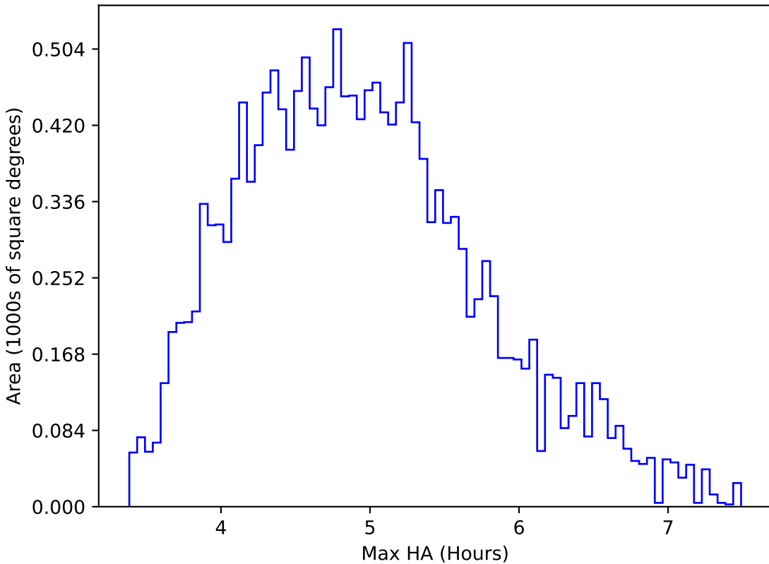
noroll_mjdp120_v3.4_10yrs WFD all bands: Max HA
